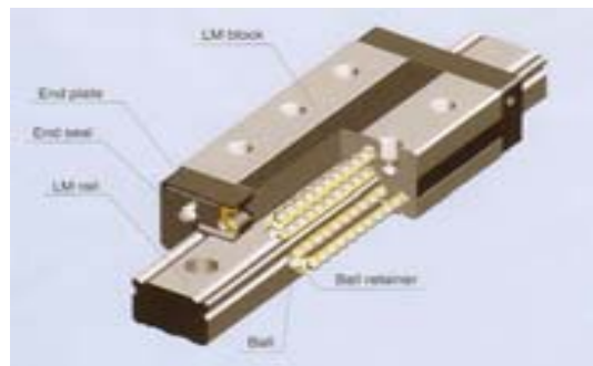
GBN uses modern Linear Bearings.
