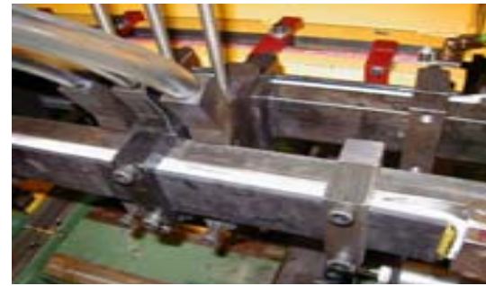
Air Clamping, no wrenches means faster changes. Compensating Chucks.
